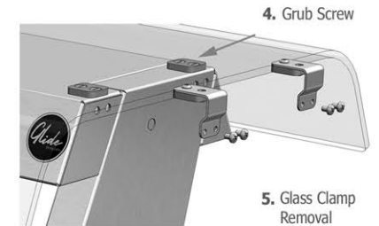
4. Grub Screw
